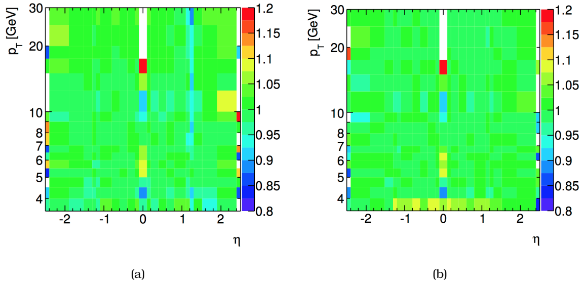
Figure 3.8: Scale factors for (a) CB and (b) ST muons.
