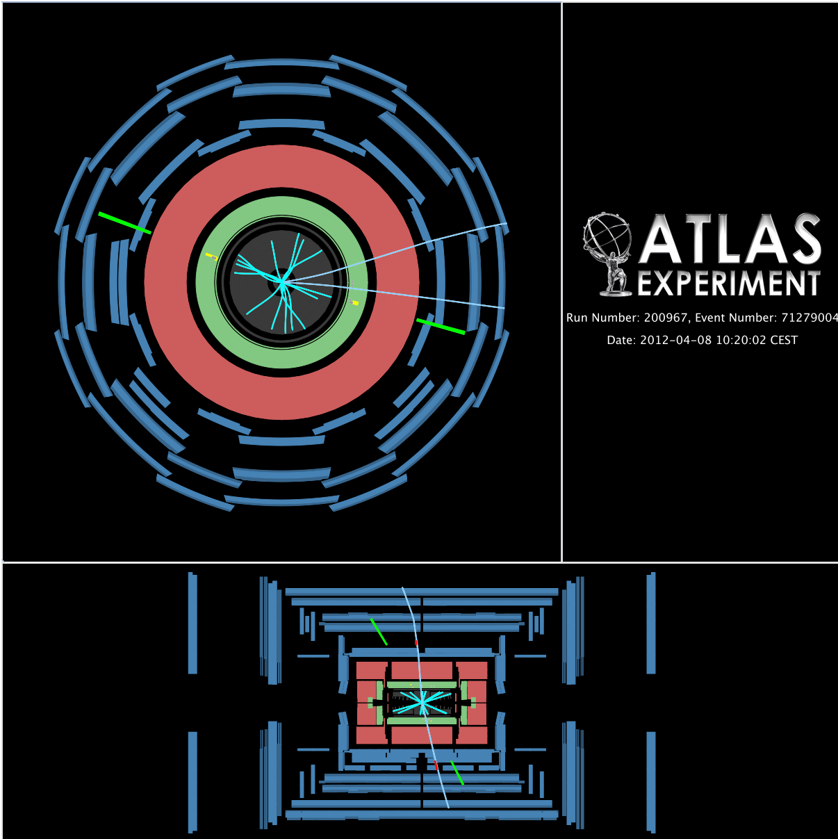
Figure 4.5: The main event display for event 71279004 in run 200967. Z electrons have p_{\text{T}}^{e_1} = 41 \text{ GeV} , p_{\text{T}}^{e_2} = 36 \text{ GeV} and \eta^{e_1} = -0.6 , \eta^{e_2} = 0.5 ( e_1 pointing at 10 o'clock and e_2 at 4 o'clock). J/\psi muons have p_{\text{T}}^{\mu_1} = 9 \text{ GeV} , p_{\text{T}}^{\mu_2} = 16 \text{ GeV} and \eta^{\mu_1} = -0.1 , \eta^{\mu_2} = 0.2 ( \mu_1 pointing at 2 o'clock and \mu_2 at 3 o'clock). The invariant mass of the Z boson candidate is found to be 87.2 \text{ GeV} and J/\psi 3.1 \text{ GeV} .
