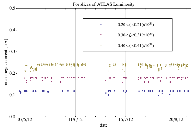
Figure 6.18: Micromegas current as a function of time for three slices of ATLAS luminosity. With the red squares luminosity is required to be between 0.30 - 0.31 \times 10^{34} \text{ cm}^{-2}\text{s}^{-1} , with blue circles between 0.20 - 0.21 \times 10^{34} \text{ cm}^{-2}\text{s}^{-1} and with the yellow triangles between 0.40 - 0.41 \times 10^{34} \text{ cm}^{-2}\text{s}^{-1} .
