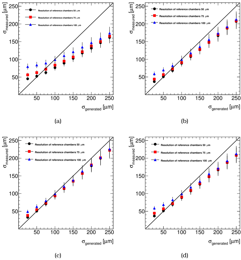
Figure 6.8: (a) Comparison of measured and generated resolution, assuming three different scenarios. With the black circles the reference detectors are modelled to have 50 \mu\text{m} resolution, with red squares 75 \mu\text{m} resolution and with blue triangles 100 \mu\text{m} resolution. The black line assumes that the generated value is equal to the measured. (b), (c), (d) Same as Figure 6.8(a), but the test chamber positioned in the alternative positions (b), (c) and (d), respectively (see Figure 6.6). The errors on all figures are multiplied by 10 in order to be visible.
